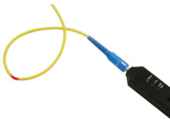
Red light from the VF 610 is visible at bends or breaks in up to 3mm jacketed single-mode fiber.
